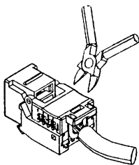
Press down the cap, and cut off extra conductor
